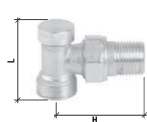
Angle lock shield valve for cooper, PEX or multilayer pipe
