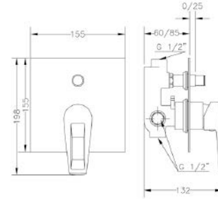
Ref.: 64116 14 45 66 Monomando de baño empotrado con inversor Built-in single lever bath mixer with diverter
