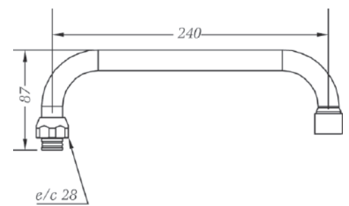
Ref.: 68902 45 Caño alto tubo 24 cm High tube spout 24 cm
