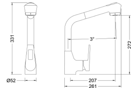
Ref.: 64206 14 45 66 Monomando de fregadera ducha extraíble Single lever sink mixer with pull-out spray
