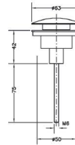
Ref.: 100202 45 Tapa universal "Click remove" "Click remove" universal cover
