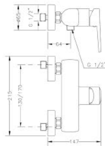
Ref.: 64110 14 45 66 Monomando de ducha con kit Single lever shower mixer with kit
