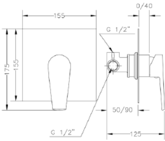
Ref.: 64115 16 45 66 Monomando de ducha empotrado Built-in single lever shower mixer
