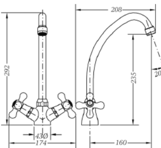
Ref.: 68540 09 45 66 Monobloc fregadera caño tubo Sink mixer, swan neck spout
