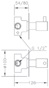
Ref.: 63114 30 45 66 Inversor cerámico 3 vías empotrado placa redonda Built-in 3 way ceramic diverter with round plate Box: 1
