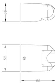
Ref.: 100068 45 Soporte ducha ovalado Oval shower holder
