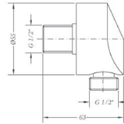
Ref.: 1680 04 Toma ducha mural redonda Round wall flexible connector
