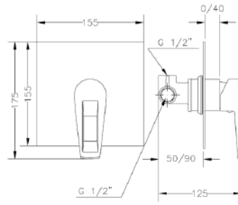
Ref.: 64115 14 45 66 Monomando de ducha empotrado Built-in single lever shower mixer
