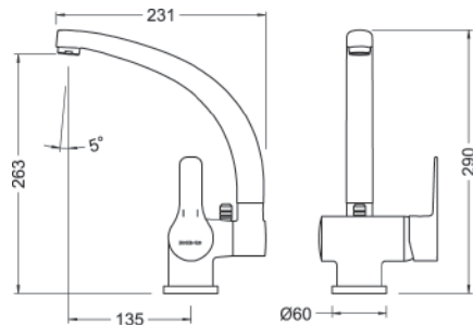
Ref.: 61900 28 45 66 Monomando de fregadera abatible Single lever folding sink mixer
