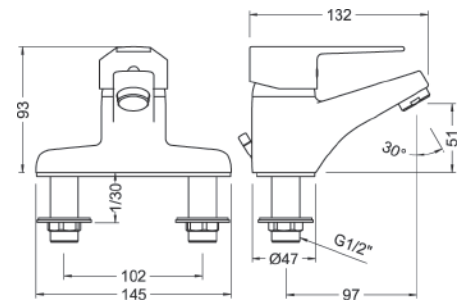
Ref.: 60188 28 45 66 Monomando de lavabo centerset 4" Single lever wash-basin mixer 4" centerset
