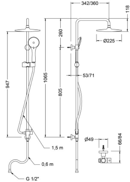
Ref.: 1744 45 Set columna fija con kit Fixed column set with kit
