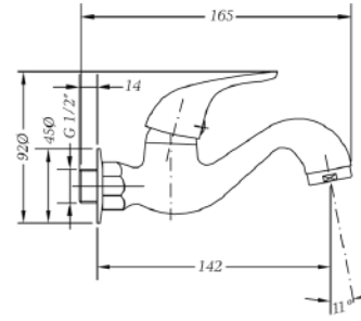
Ref.: 1006 04 Grifo lavabo mural 1 agua cartucho 25 One-water wall wash-basin tap 25 cartridge
