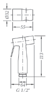
Ref.: 100694 60 Kit ducha sanitaria inox Inox sanitary shower kit
