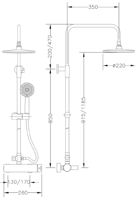
Ref.: CM65110 29 Columna monomando extensible con kit Single lever extensible column with kit
