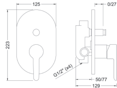
Ref.: 65116 19 45 66 Monomando de baño empotrado con inversor Built-in single lever bath mixer with diverter
