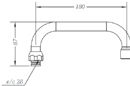
Ref.: 68901 45 Caño alto tubo 18 cm High tube spout 18 cm
