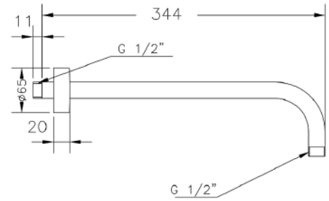
Ref.: B65114 18 Brazo pared redondo 24 cm Round arm 24 cm
