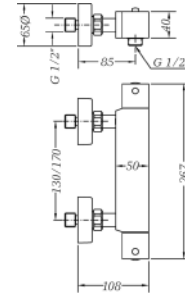
Ref.: 67110 26 45 67 Termostática ducha sin kit Thermostatic shower mixer without kit
