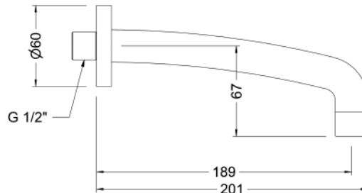
Ref.: 68913 45 Caño mural tubo inclinado 20 cm Wall mounted sloping pipe spout 20 cm
