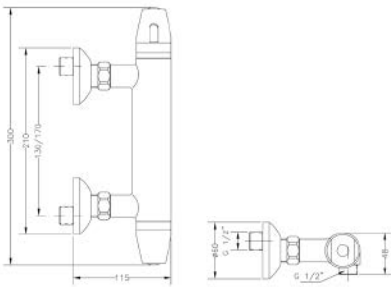
Ref.: 67104 14 45 67 Termostática ducha Thermostatic shower mixer
