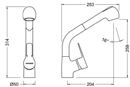
Ref.: 61206 28 45 66 Monomando de fregadera ducha extraíble Single-lever sink mixer with pull-out spray
