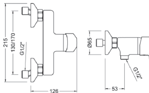
Ref.: 60110 28 45 66 Monomando de ducha con kit Single lever shower mixer with kit
