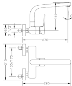
Ref.: 64192 16 45 66 Monomando de fregadera mural Wall single lever sink mixer
