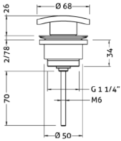
Ref.: 100204 45 Válvula click Kenjo 1 1/4" 1 1/4" Kenjo click valve
