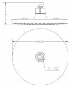
Ref.: R65112 18 Rociador redondo 22 cm Round shower head 22 cm
