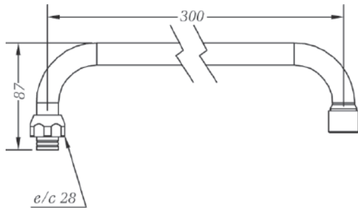
Ref.: 68908 45 Caño alto tubo 30 cm High tube spout 30 cm
