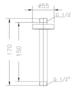
Ref.: 1671 45 Brazo a techo redondo 15 cm Round roof arm 15 cm
