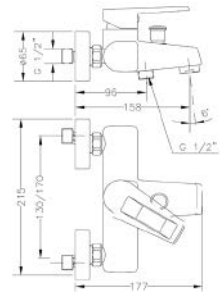
Ref.: 64100 14 45 66 Monomando de baño con kit Single lever bath mixer with kit
