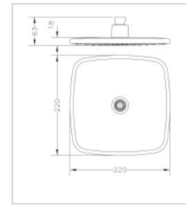
Ref.: R63112 08 Rociador ovalado 22 cm Oval shower head 22 cm
