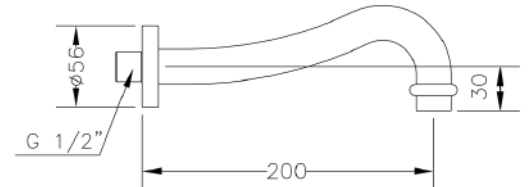
Ref.: 68914 45 Caño mural tubo retro 20 cm Wall mounted retro pipe spout 20 cm
