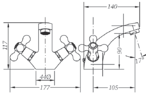
Ref.: 68505 09 45 66 Monobloc de lavabo Wash-basin mixer
