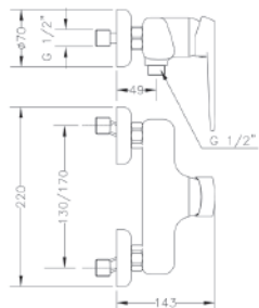
Ref.: 62110 31 45 67 Monomando de ducha sin kit Single lever shower mixer without kit
