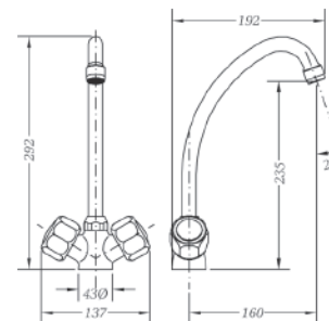
Ref.: 68200 11 45 66 Monobloc de fregadera caño tubo Sink mixer, swan neck spout
