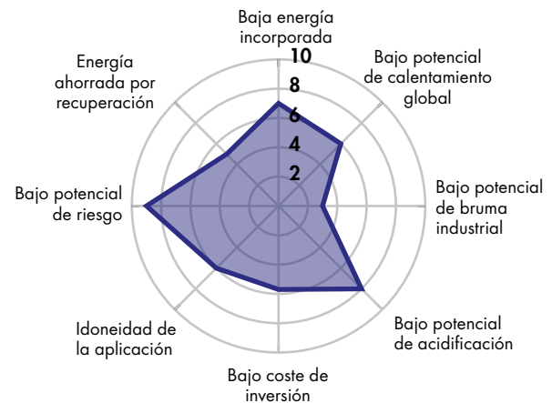
PUR/PIR 12 cm
