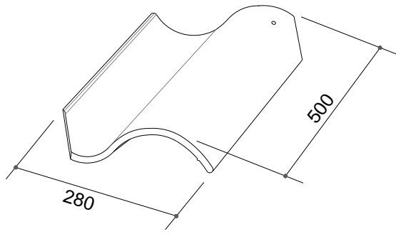
TEJA VEREA SPANISH S
